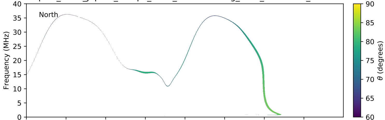
expres_earth_jupiter_europa_isaac_lossc-wid1deg_3kev_20171127_v01.cdf
