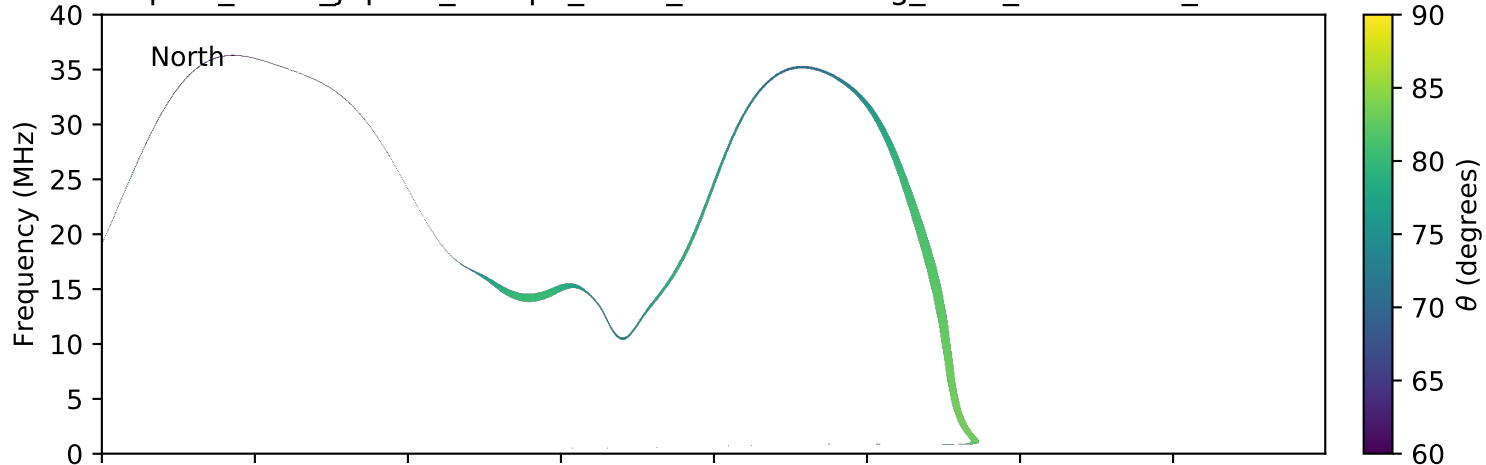
expres_earth_jupiter_europa_isaac_lossc-wid1deg_3kev_20171120_v01.cdf
