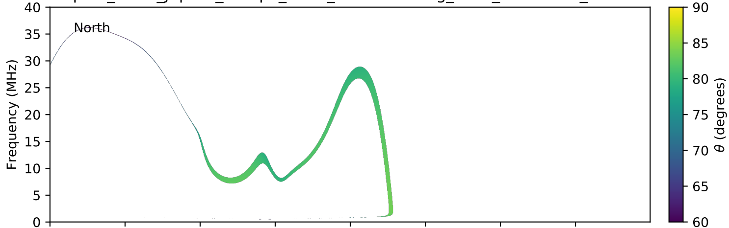
expres_earth_jupiter_europa_isaac_lossc-wid1deg_3kev_20171106_v01.cdf
