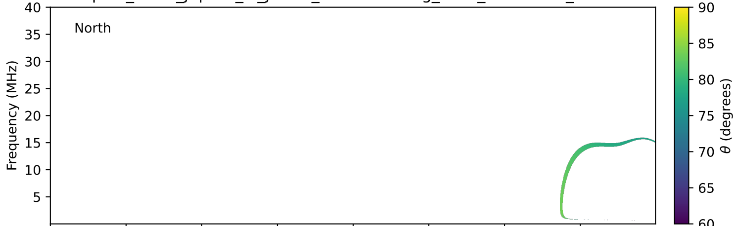
expres_earth_jupiter_io_jrm33_lossc-wid1deg_3kev_20170929_v11.cdf
