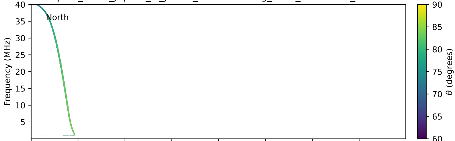
expres_earth_jupiter_io_jrm33_lossc-wid1deg_3kev_20170927_v11.cdf
