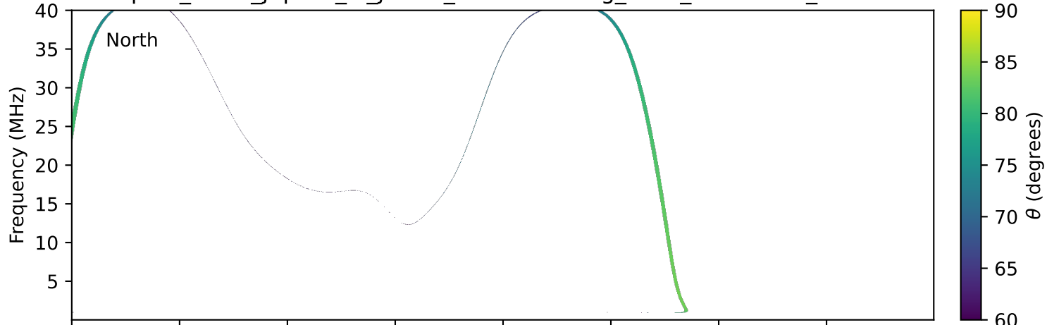
expres_earth_jupiter_io_jrm33_lossc-wid1deg_3kev_20170914_v11.cdf
