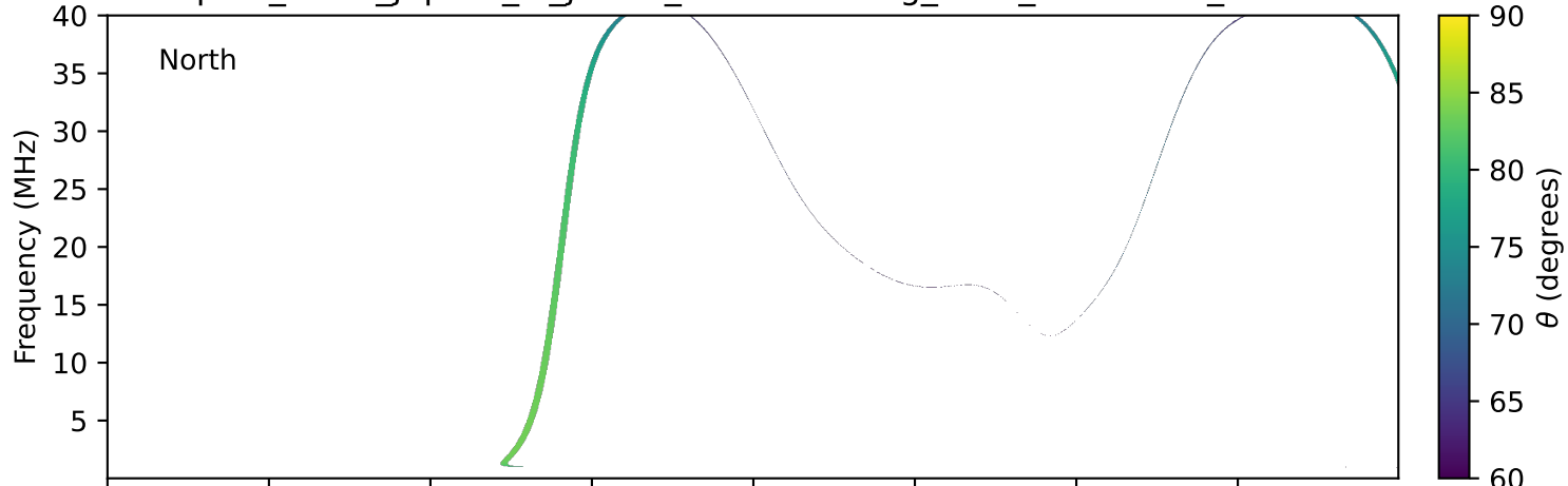
expres_earth_jupiter_io_jrm33_lossc-wid1deg_3kev_20170912_v11.cdf
