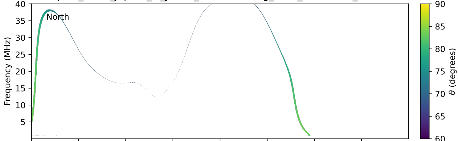
expres_earth_jupiter_io_jrm33_lossc-wid1deg_3kev_20170907_v11.cdf
