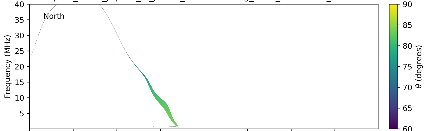
expres_earth_jupiter_io_jrm33_lossc-wid1deg_3kev_20170902_v11.cdf
