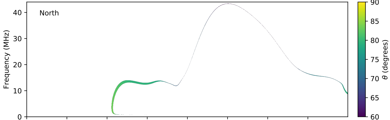
expres_earth_jupiter_io_jrm09_lossc-wid1deg_3kev_20170930_v01.cdf
