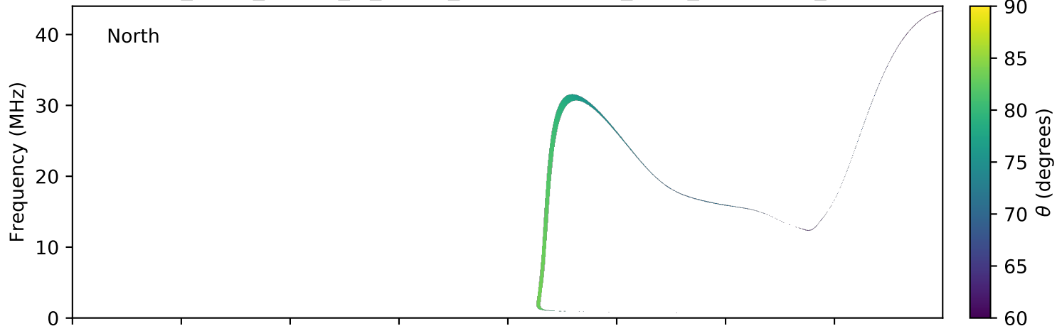
expres_earth_jupiter_io_jrm09_lossc-wid1deg_3kev_20170928_v01.cdf
