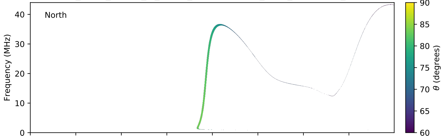
expres_earth_jupiter_io_jrm09_lossc-wid1deg_3kev_20170921_v01.cdf
