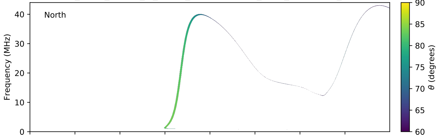
expres_earth_jupiter_io_jrm09_lossc-wid1deg_3kev_20170914_v01.cdf
