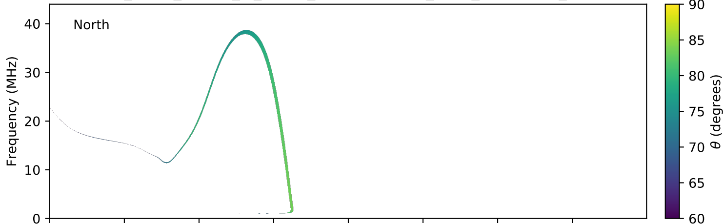
expres_earth_jupiter_io_jrm09_lossc-wid1deg_3kev_20170913_v01.cdf
