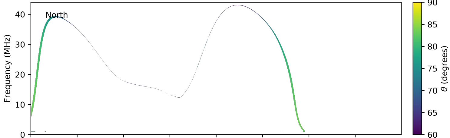
expres_earth_jupiter_io_jrm09_lossc-wid1deg_3kev_20170902_v01.cdf
