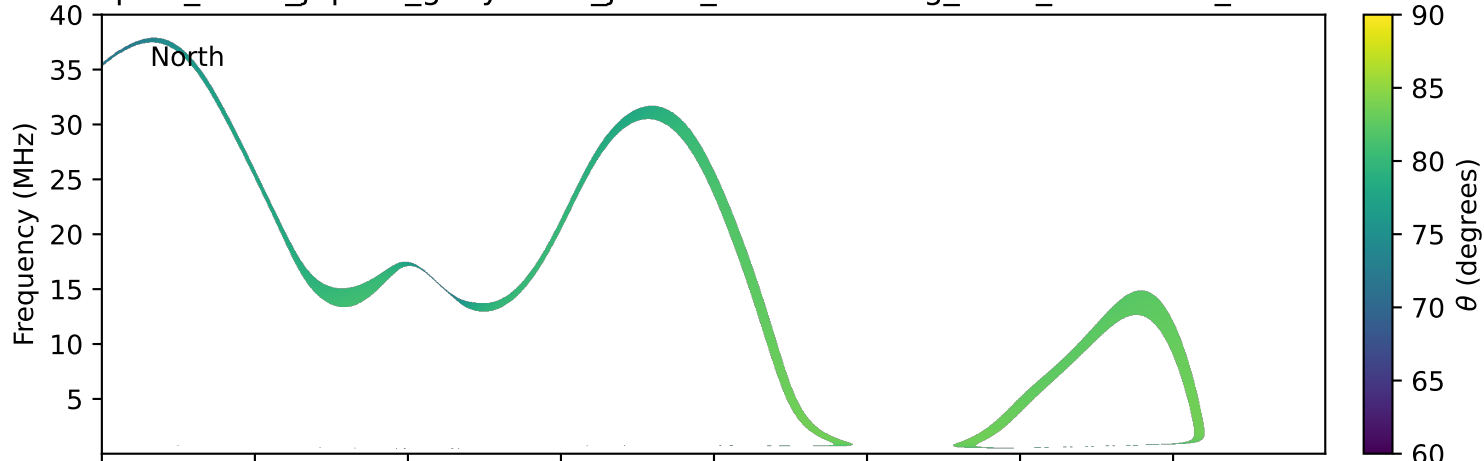
expres_earth_jupiter_ganymede_jrm33_lossc-wid1deg_3kev_20170910_v11.cdf
