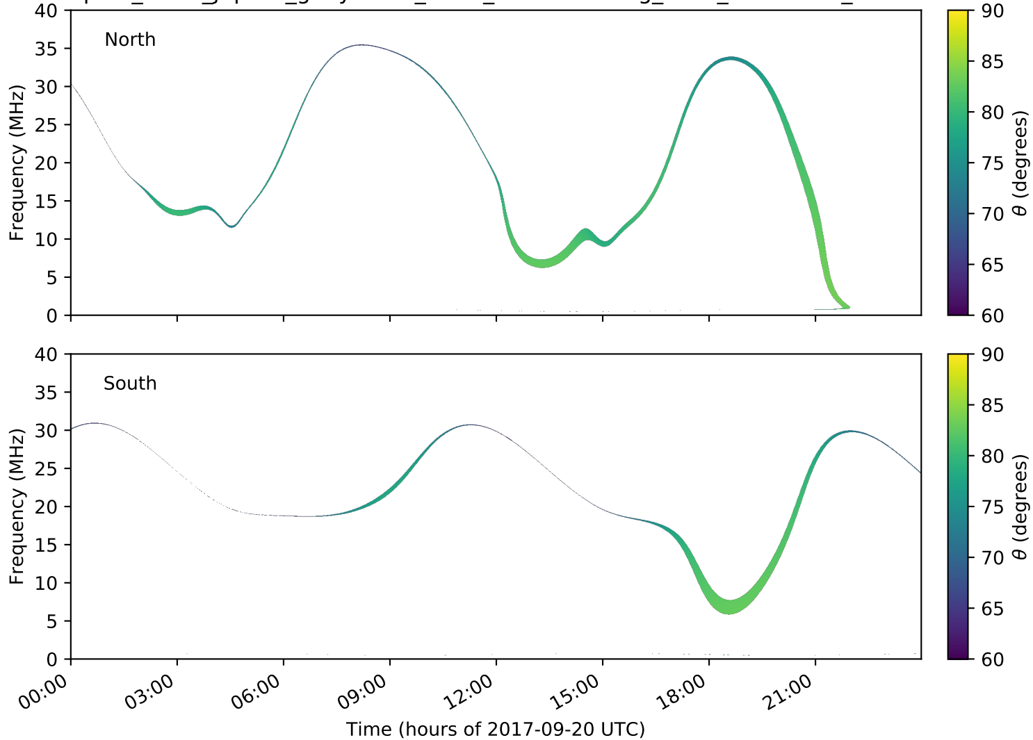
expres_earth_jupiter_ganymede_isaac_lossc-wid1deg_3kev_20170920_v01.cdf
