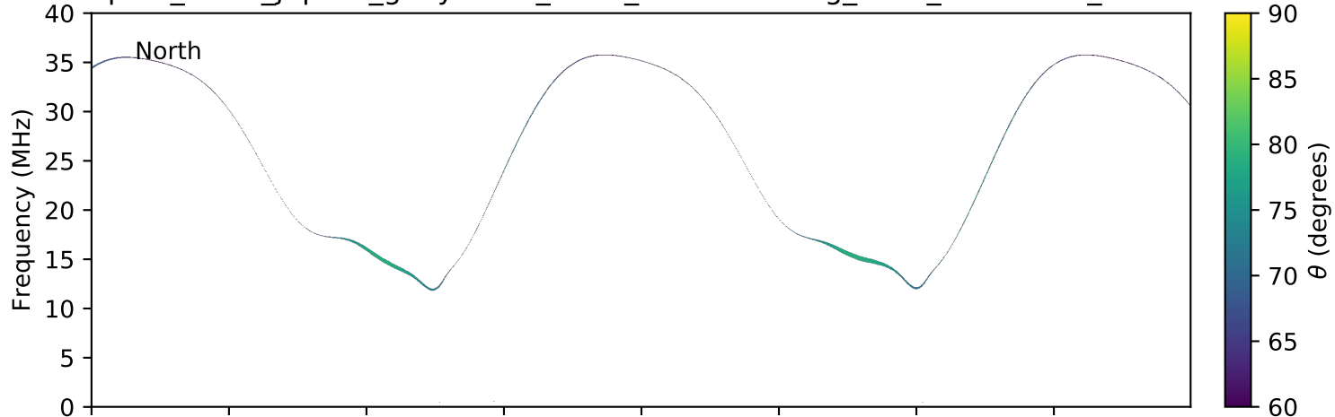
expres_earth_jupiter_ganymede_isaac_lossc-wid1deg_3kev_20170919_v01.cdf
