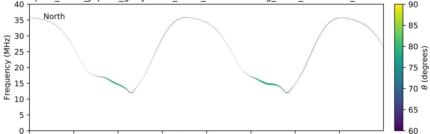
expres_earth_jupiter_ganymede_isaac_lossc-wid1deg_3kev_20170912_v01.cdf
