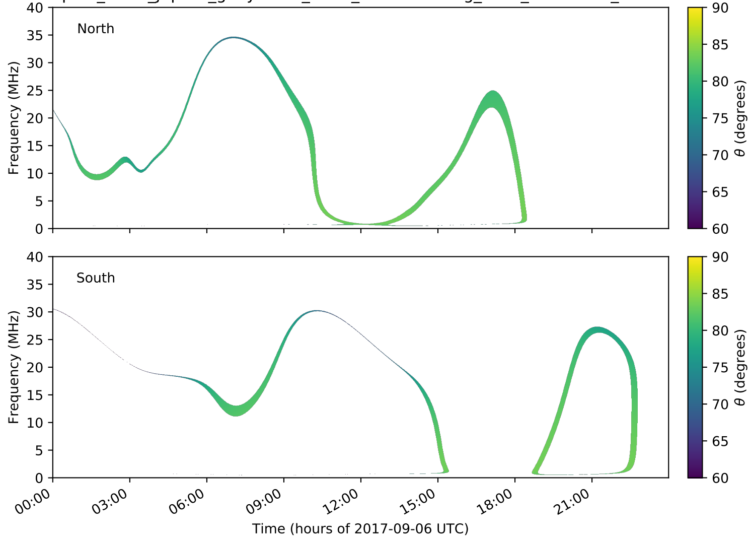
expres_earth_jupiter_ganymede_isaac_lossc-wid1deg_3kev_20170906_v01.cdf
