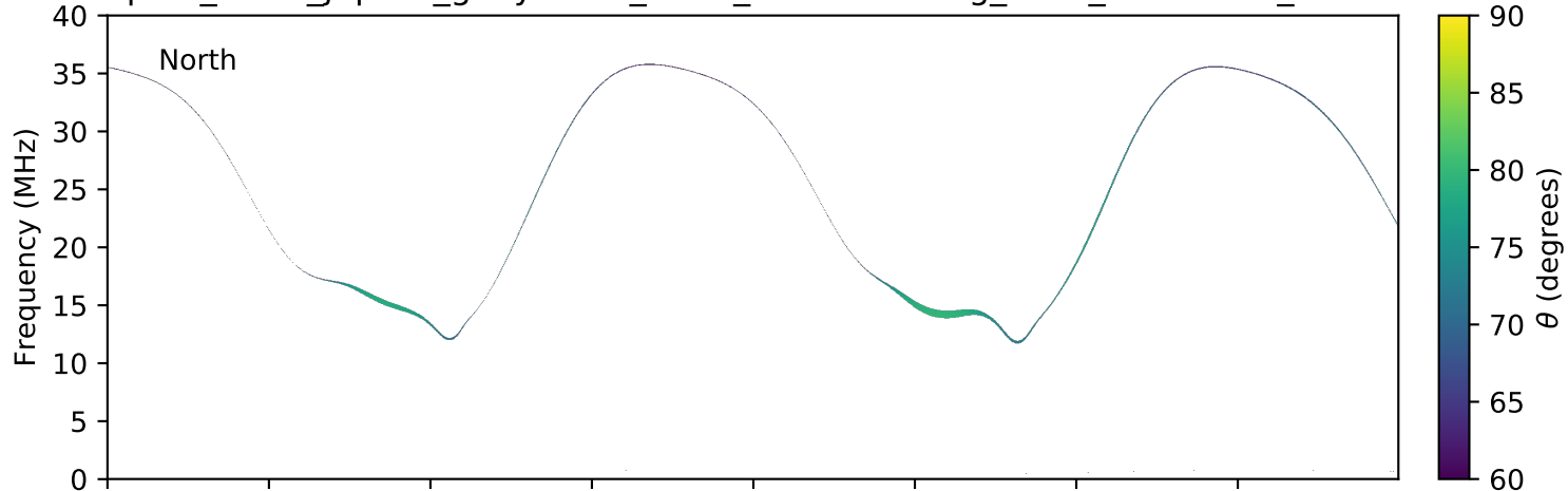
expres_earth_jupiter_ganymede_isaac_lossc-wid1deg_3kev_20170905_v01.cdf
