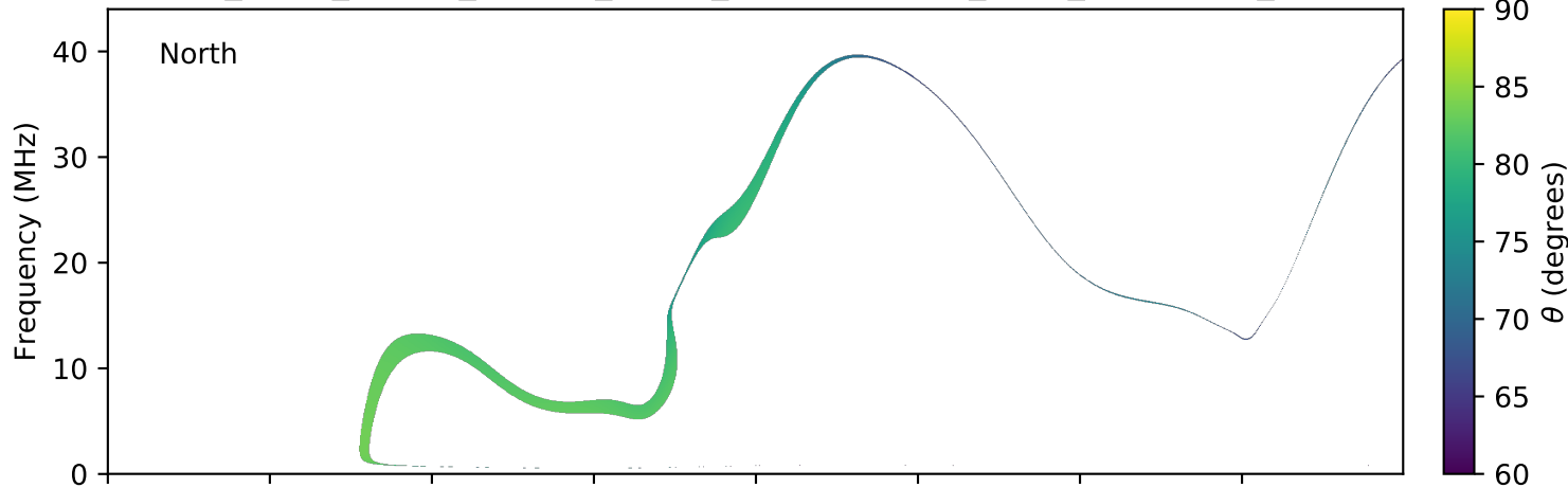
expres_earth_jupiter_europa_jrm09_lossc-wid1deg_3kev_20170923_v01.cdf
