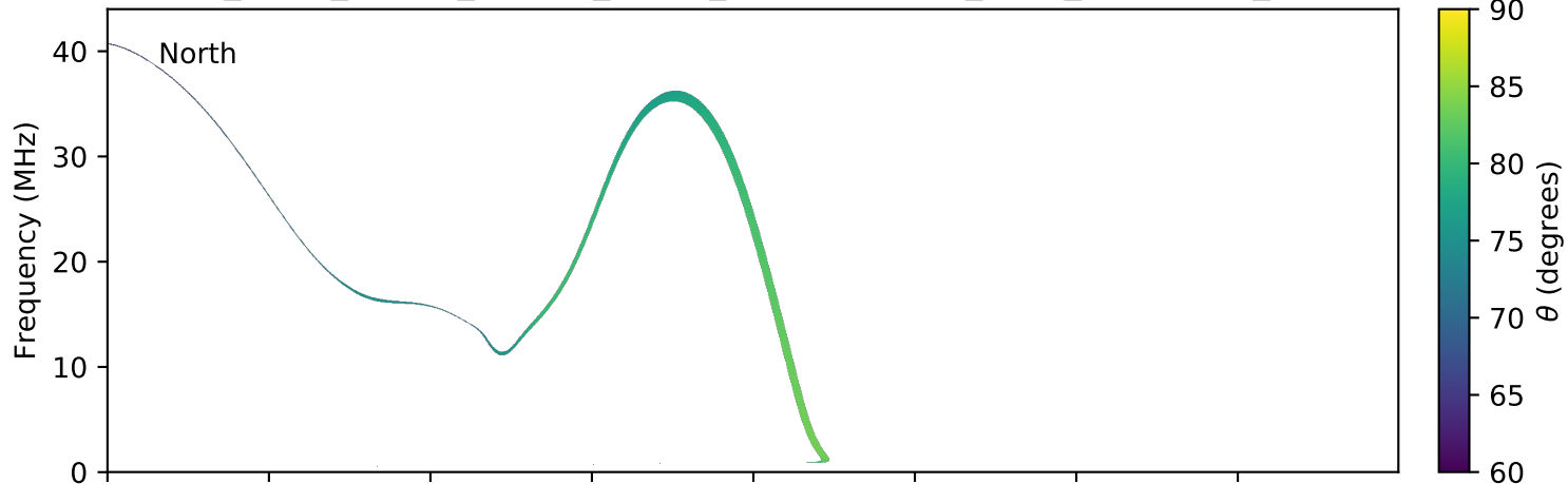
expres_earth_jupiter_europa_jrm09_lossc-wid1deg_3kev_20170910_v01.cdf
