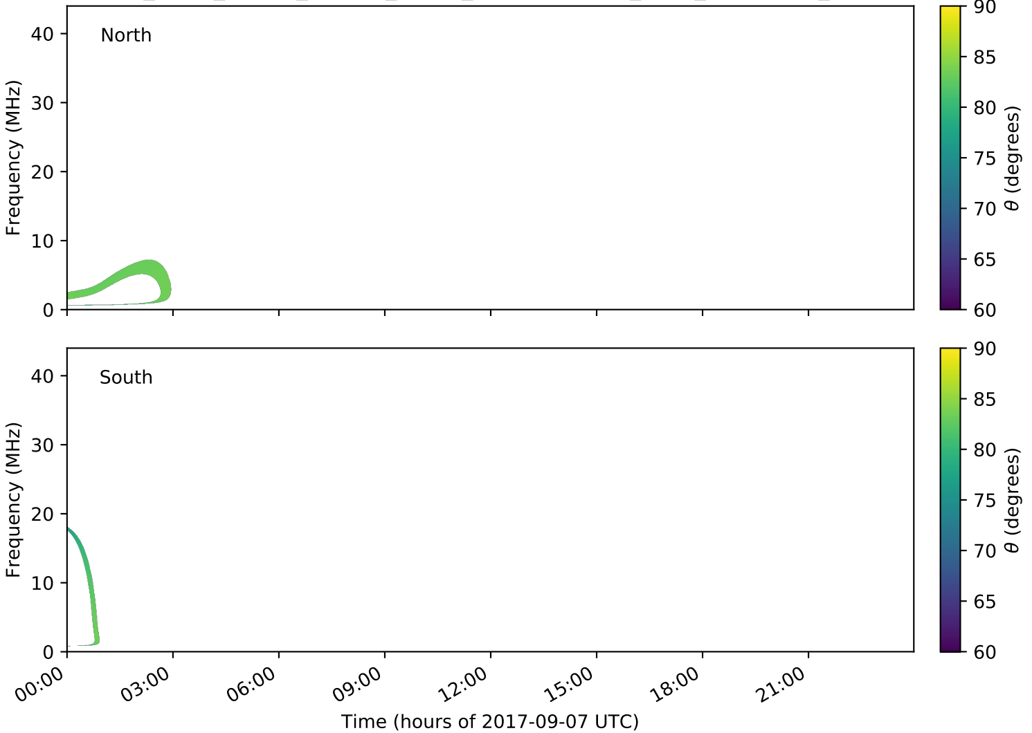
expres_earth_jupiter_europa_jrm09_lossc-wid1deg_3kev_20170907_v01.cdf
