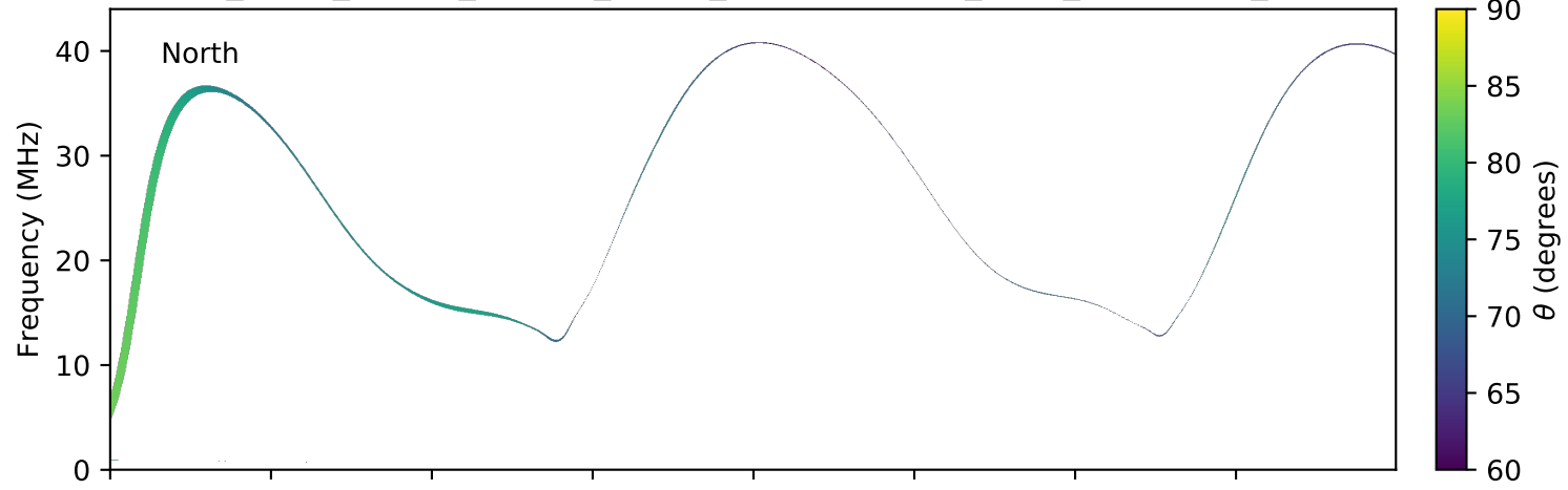
expres_earth_jupiter_europa_jrm09_lossc-wid1deg_3kev_20170902_v01.cdf
