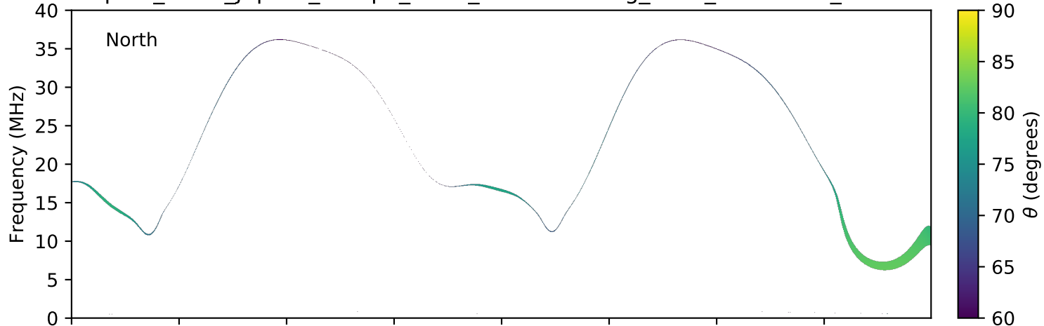
expres_earth_jupiter_europa_isaac_lossc-wid1deg_3kev_20170913_v01.cdf
