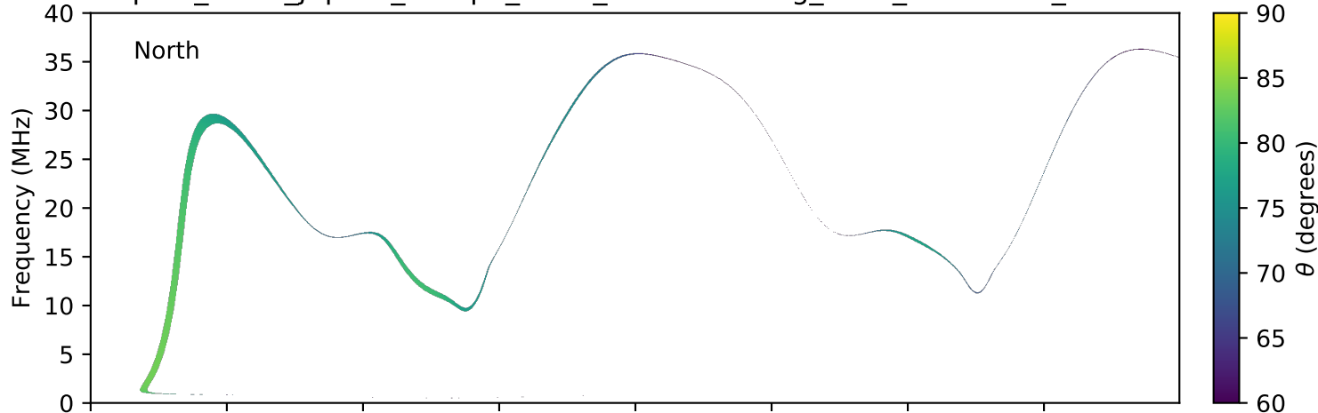
expres_earth_jupiter_europa_isaac_lossc-wid1deg_3kev_20170909_v01.cdf
