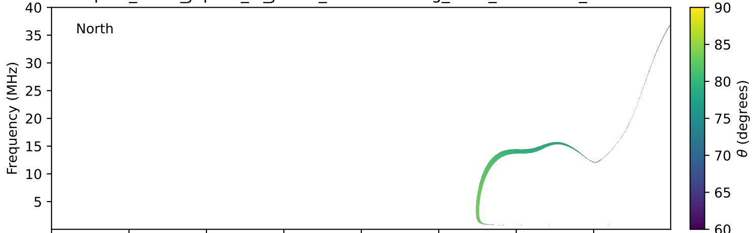
expres_earth_jupiter_io_jrm33_lossc-wid1deg_3kev_20170825_v11.cdf
