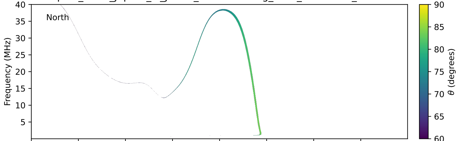
expres_earth_jupiter_io_jrm33_lossc-wid1deg_3kev_20170819_v11.cdf
