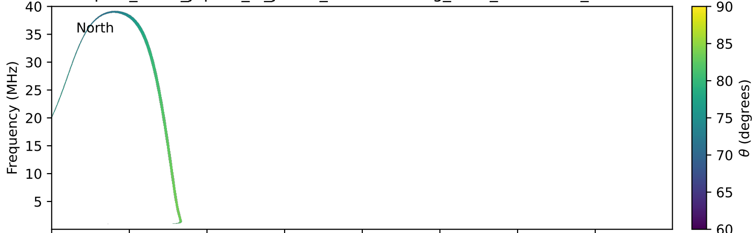
expres_earth_jupiter_io_jrm33_lossc-wid1deg_3kev_20170807_v11.cdf
