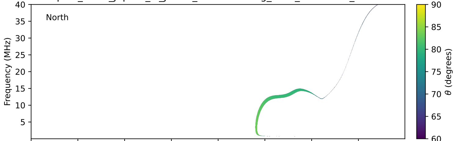
expres_earth_jupiter_io_jrm33_lossc-wid1deg_3kev_20170804_v11.cdf
