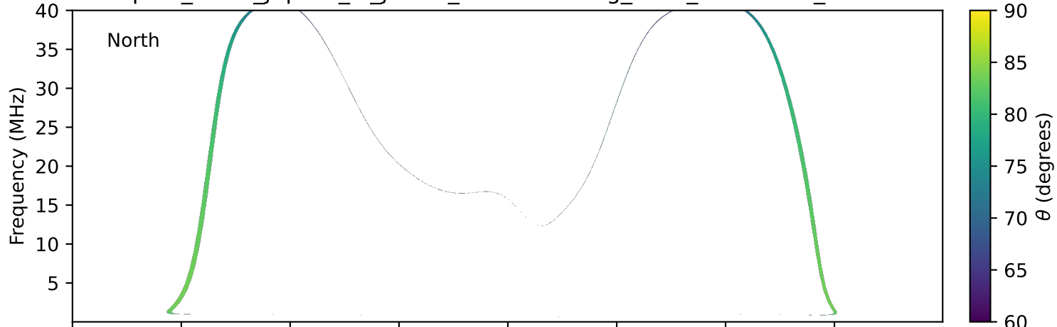
expres_earth_jupiter_io_jrm33_lossc-wid1deg_3kev_20170801_v11.cdf
