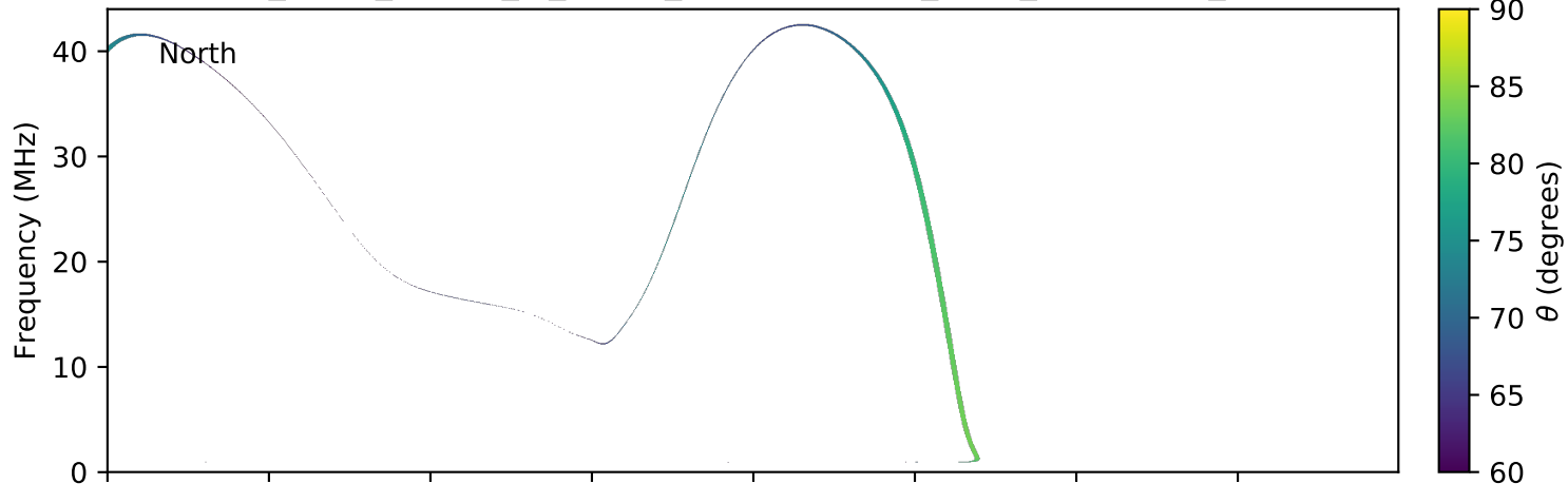
expres_earth_jupiter_io_jrm09_lossc-wid1deg_3kev_20170826_v01.cdf
