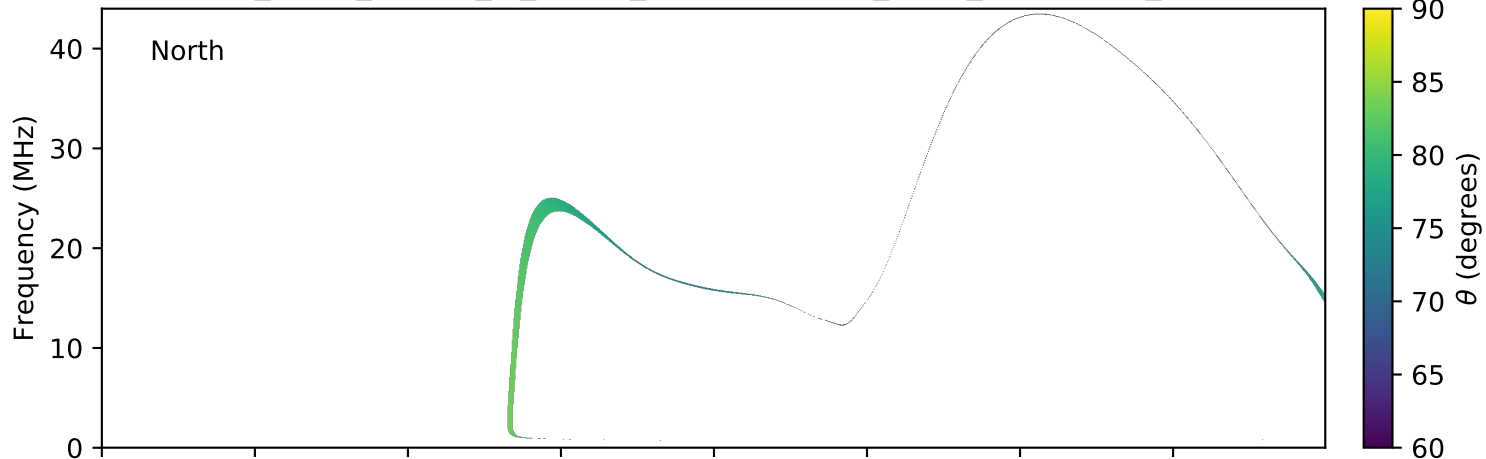
expres_earth_jupiter_io_jrm09_lossc-wid1deg_3kev_20170822_v01.cdf
