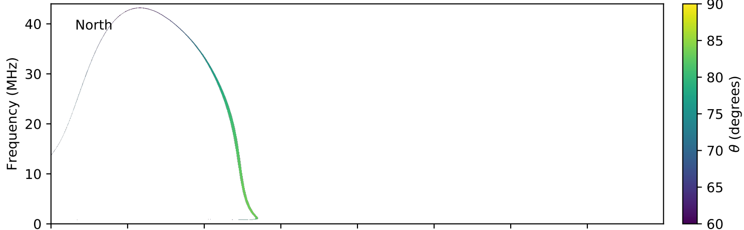
expres_earth_jupiter_io_jrm09_lossc-wid1deg_3kev_20170821_v01.cdf
