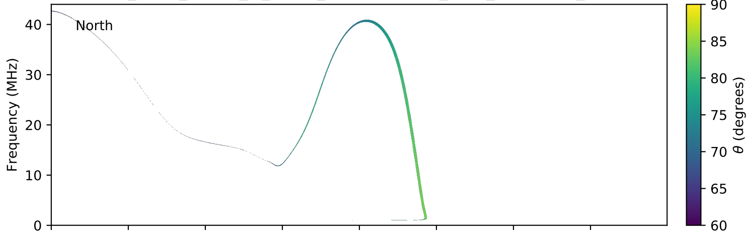
expres_earth_jupiter_io_jrm09_lossc-wid1deg_3kev_20170819_v01.cdf
