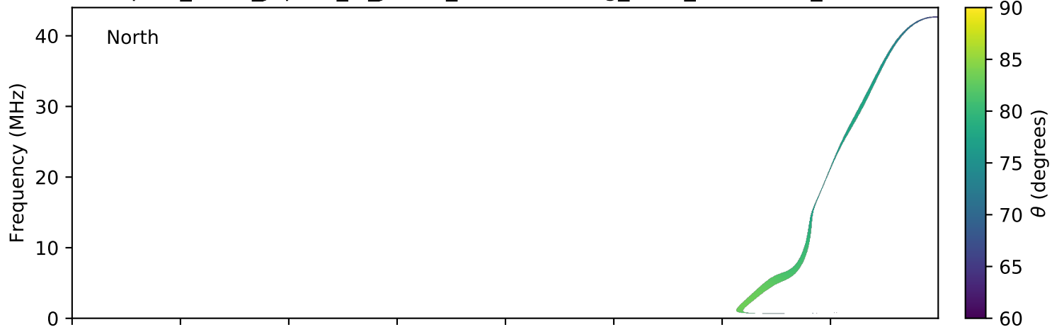
expres_earth_jupiter_io_jrm09_lossc-wid1deg_3kev_20170818_v01.cdf
