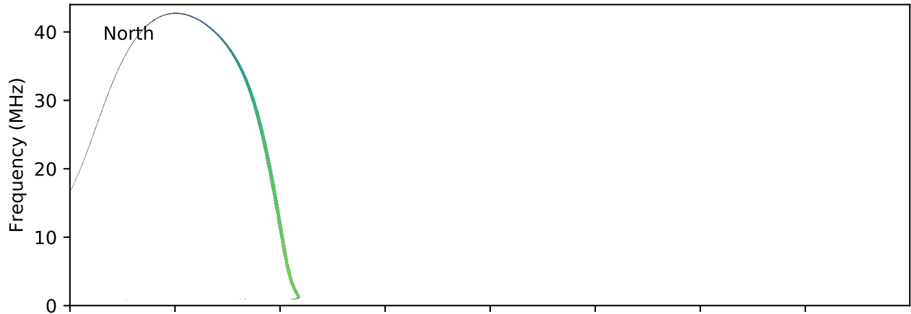
expres_earth_jupiter_io_jrm09_lossc-wid1deg_3kev_20170814_v01.cdf
