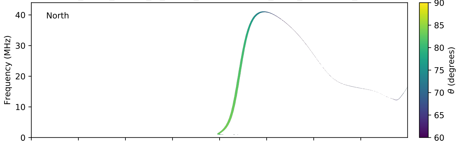
expres_earth_jupiter_io_jrm09_lossc-wid1deg_3kev_20170813_v01.cdf
