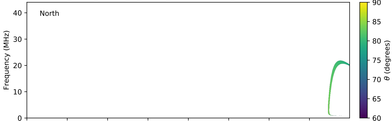
expres_earth_jupiter_io_jrm09_lossc-wid1deg_3kev_20170809_v01.cdf
