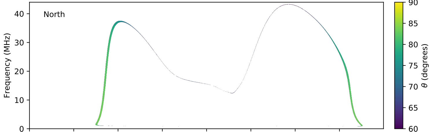
expres_earth_jupiter_io_jrm09_lossc-wid1deg_3kev_20170808_v01.cdf
