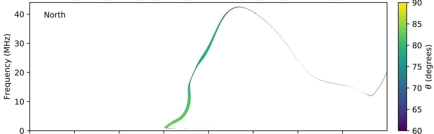
expres_earth_jupiter_io_jrm09_lossc-wid1deg_3kev_20170806_v01.cdf
