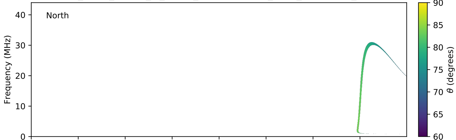
expres_earth_jupiter_io_jrm09_lossc-wid1deg_3kev_20170802_v01.cdf
