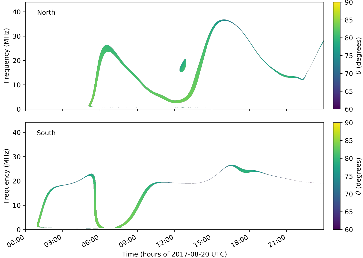
expres_earth_jupiter_ganymede_jrm09_lossc-wid1deg_3kev_20170820_v01.cdf
