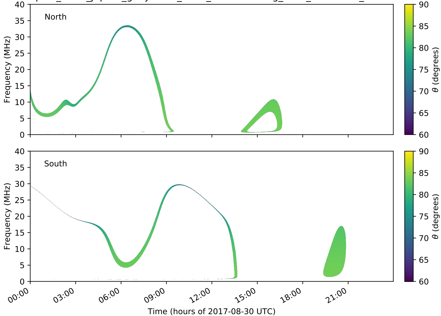
expres_earth_jupiter_ganymede_isaac_lossc-wid1deg_3kev_20170830_v01.cdf
