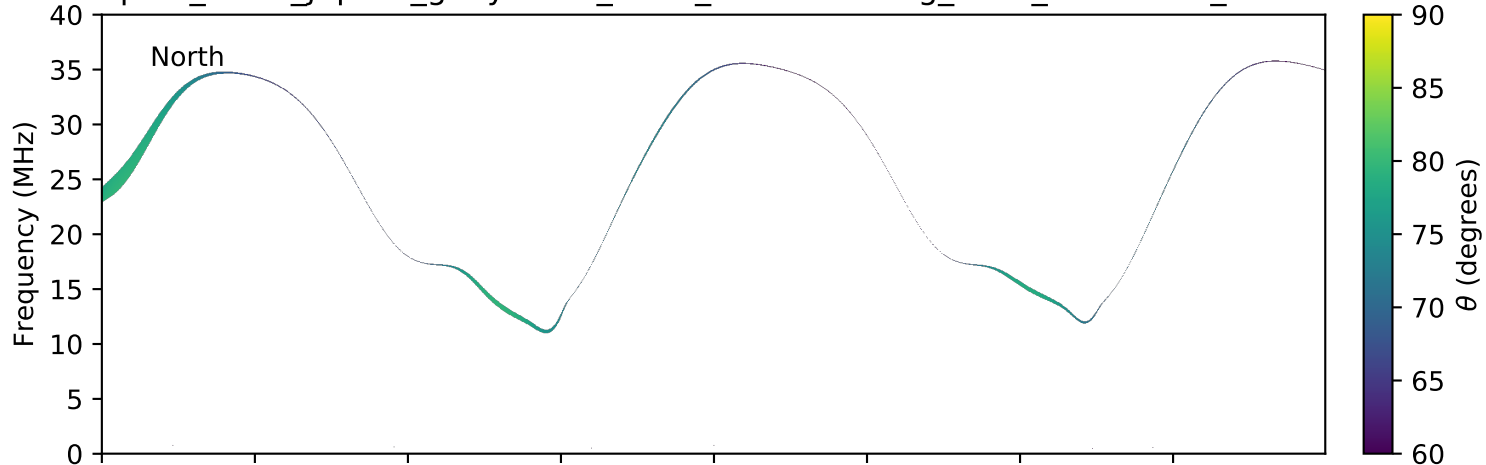
expres_earth_jupiter_ganymede_isaac_lossc-wid1deg_3kev_20170828_v01.cdf
