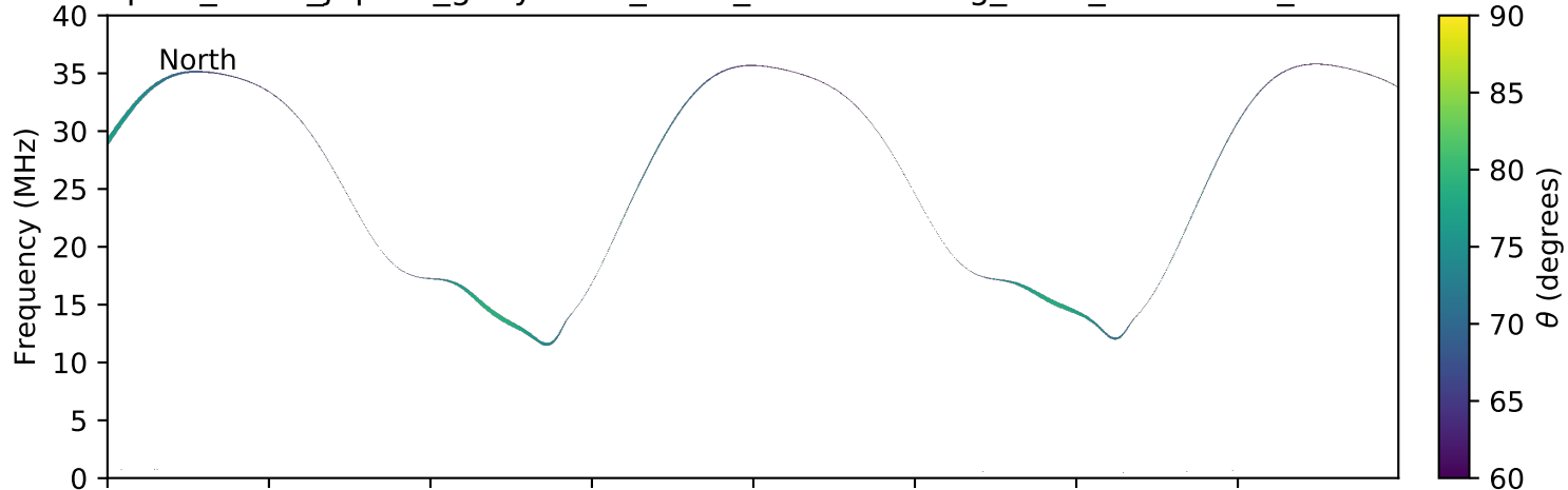
expres_earth_jupiter_ganymede_isaac_lossc-wid1deg_3kev_20170821_v01.cdf
