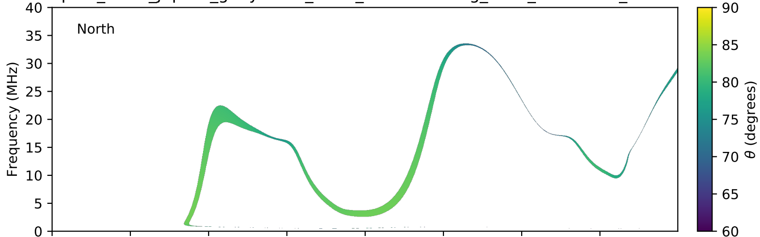
expres_earth_jupiter_ganymede_isaac_lossc-wid1deg_3kev_20170820_v01.cdf
