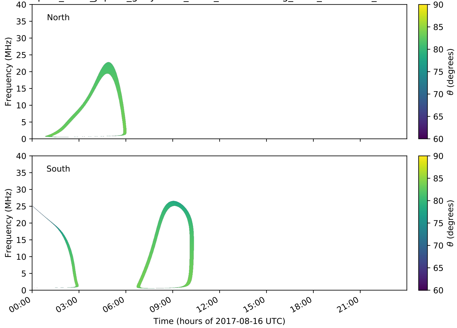
expres_earth_jupiter_ganymede_isaac_lossc-wid1deg_3kev_20170816_v01.cdf
