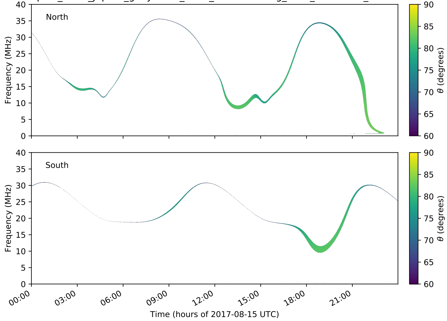
expres_earth_jupiter_ganymede_isaac_lossc-wid1deg_3kev_20170815_v01.cdf
